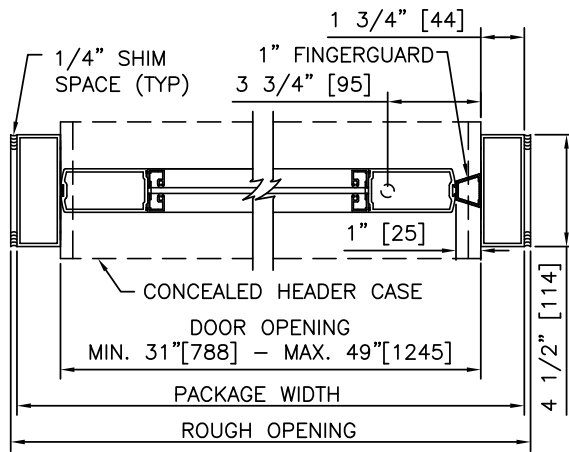
2 HORIZONTAL SECTION
